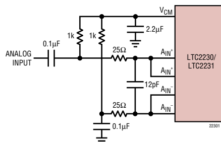
Figure 5. Single-Ended Drive
