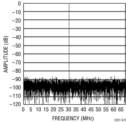
LTC2231: 8192 Point FFT, f_{IN} = 30\text{MHz} , -1\text{dB} , 1\text{V} Range
